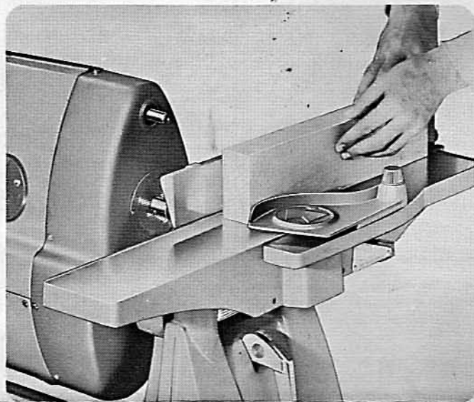
4" MAGNA JOINTER ON SHOPSMITH. Shown above: Feeding workpiece into Jointer. The 3 Jointer knives are precision-ground . . . are tapered to seat against matching retaining wedges for maximum safety.
