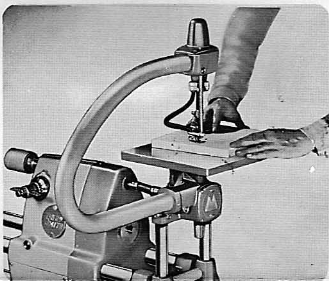
18" MAGNA JIGSAW ON SHOPSMITH. Shown above: Jigsaw on Power Mount, with Drum Sander on front spindle for sanding finished contours of work done on jigsaw.
